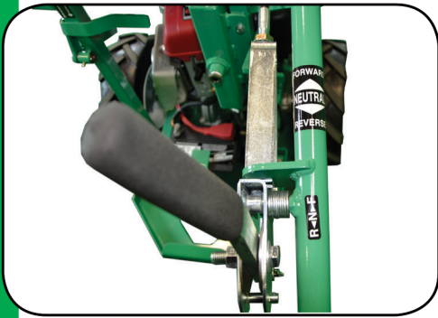
Hydrostatic Drive with handlebar mounted forward/reverse lever.
